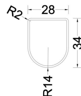
(床换截面尺寸图)
