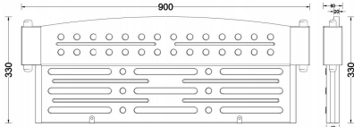
(边立柱床挡护栏规格图)
