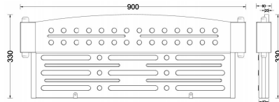
(边立柱床挡护栏规格图)
