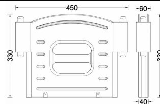
(中立柱床挡规格图)
