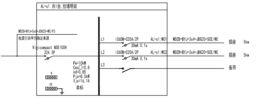
AL-s1配电箱
