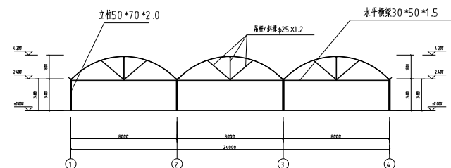
1a~a剖面图
